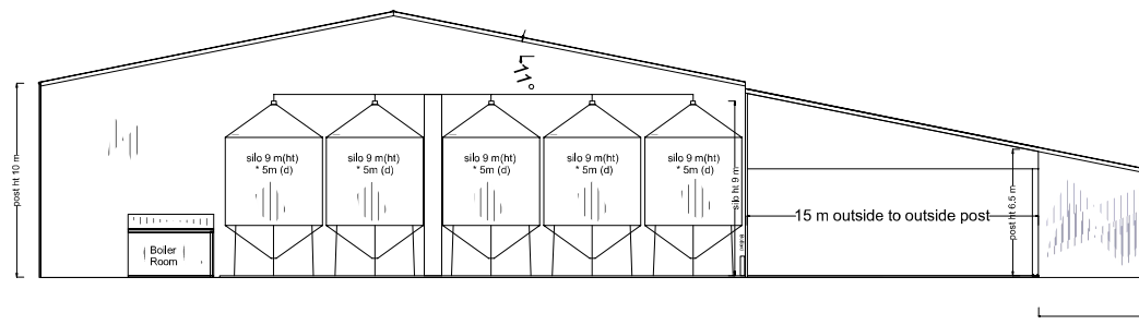
Eastern Elevation
